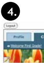
Figure 5: Logout Button
