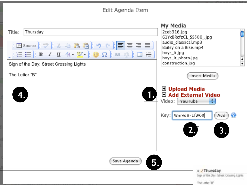
Figure 1: Editor Window
